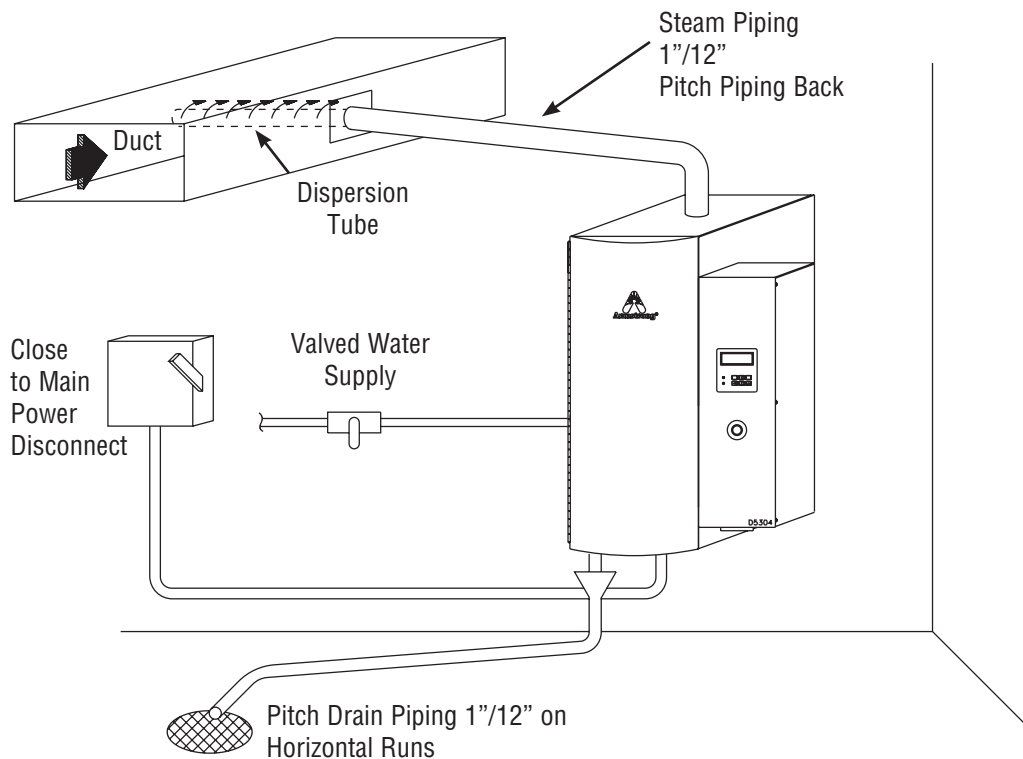
Figure 148-2. HC-6100 or HC-6300 General Installation Concept
